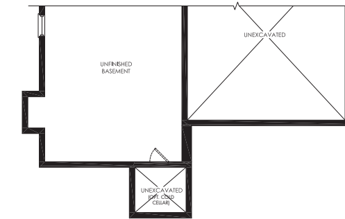
PARTIAL BASEMENT PLAN ELEV. 'B'
