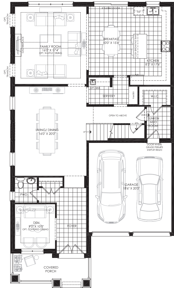
GROUND FLOOR PLAN ELEV. 'A'
