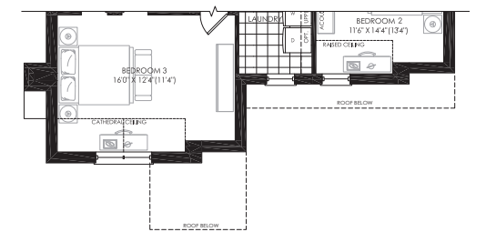
PARTIAL SECOND FLOOR PLAN ELEV. 'D'
